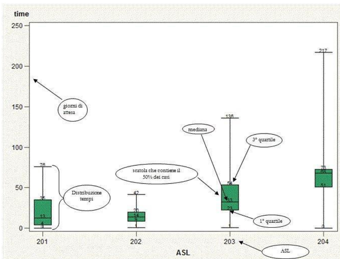
Figura 1: box plot
